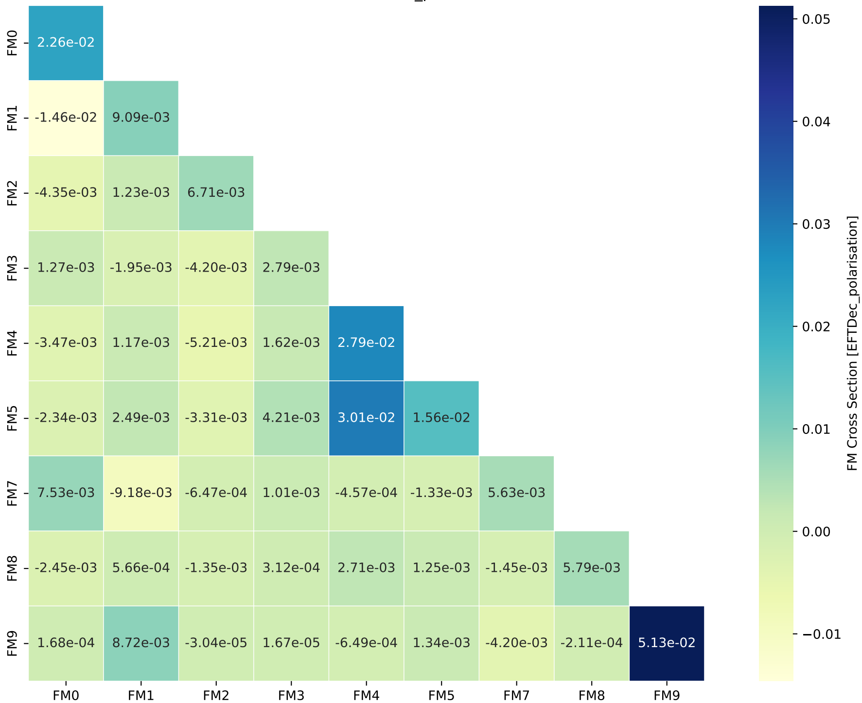
FM Cross Section [EFTDec_polarisation]
